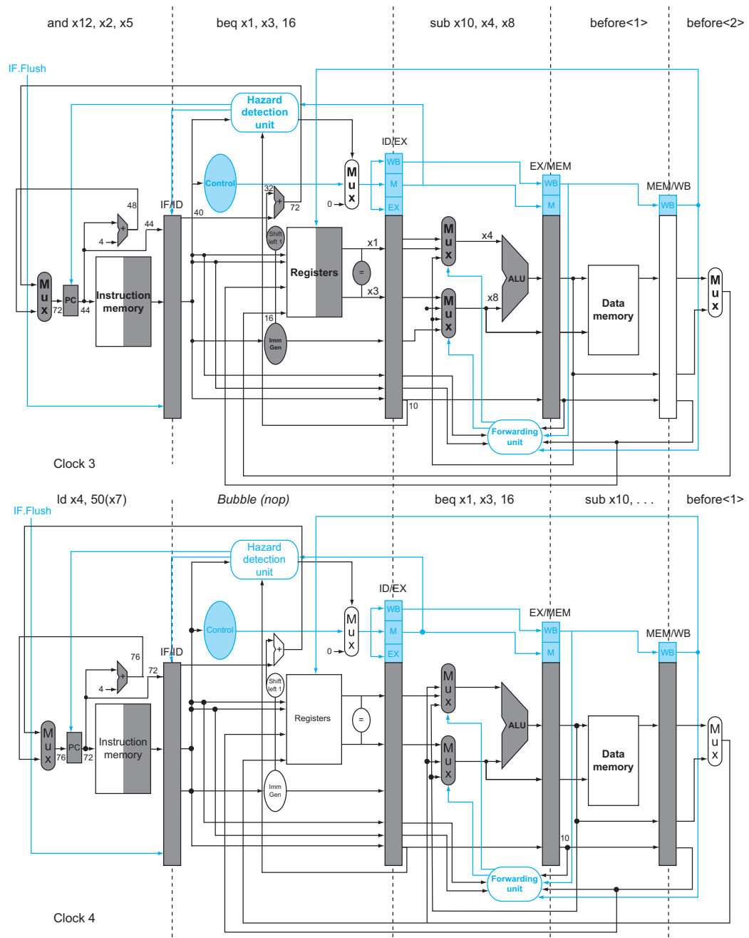
FIGURE 4.60 The ID stage of clock cycle 3 determines that a branch must be taken, so it selects 72 as the next PC address and zeros the instruction fetched for the next clock cycle. Clock cycle 4 shows the instruction at location 72 being fetched and the single bubble or nop instruction in the pipeline because of the taken branch.
