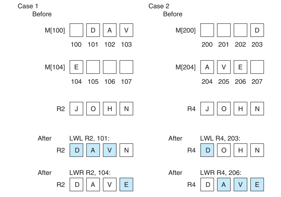
FIGURE D.7.1 MIPS instructions for unaligned word reads. This figure assumes operation in big-endian mode. Case 1 first loads the three bytes 101, 102, and 103 into the left of R2, leaving the least significant byte undisturbed. The following LWR simply loads byte 104 into the least significant byte of R2, leaving the other bytes of the register unchanged using LWL. Case 2 first loads byte 203 into the most significant byte of R4, and the following LWR loads the other three bytes of R4 from memory bytes 204, 205, and 206. LWL reads the word with the first byte from memory, shifts to the left to discard the unneeded byte(s), and changes only those bytes in Rd. The byte(s) transferred are from the first byte to the lowest-order byte of the word. The following LWR addresses the last byte, right-shifts to discard the unneeded byte(s), and finally changes only those bytes of Rd. The byte(s) transferred are from the last byte up to the highest-order byte of the word. Store word left (SWL) is simply the inverse of LWL, and store word right (SWR) is the inverse of LWR. Changing to little-endian mode flips which bytes are selected and discarded. (If big-little, left-right, load-store seem confusing, don't worry; they work!)
