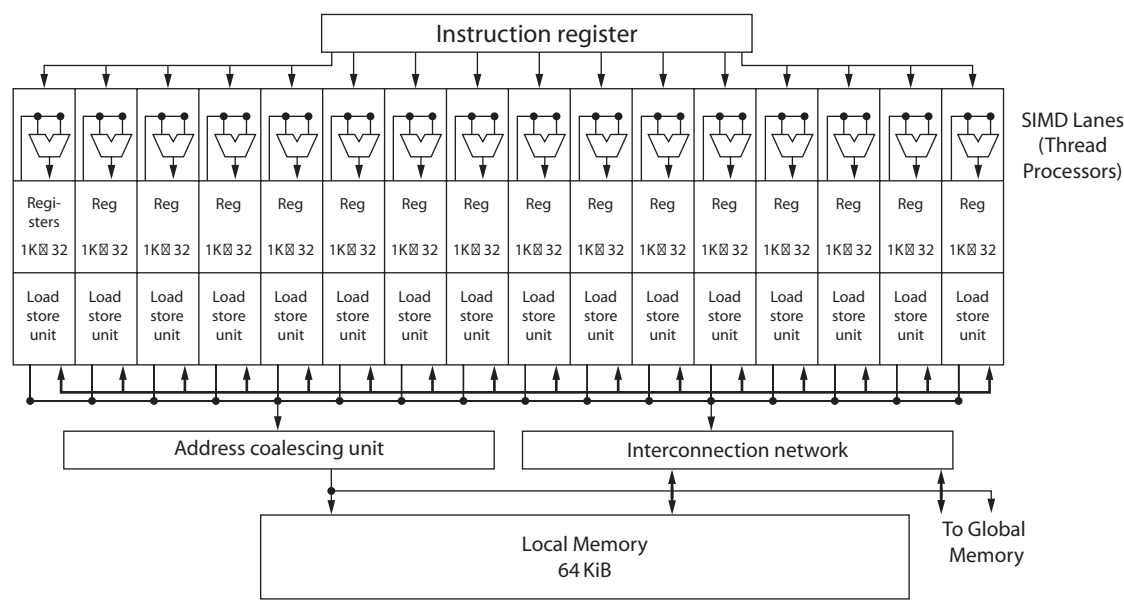
FIGURE 6.9 Simplified block diagram of the datapath of a multithreaded SIMD Processor. It has 16 SIMD lanes. The SIMD Thread Scheduler has many independent SIMD threads that it chooses from to run on this processor.
