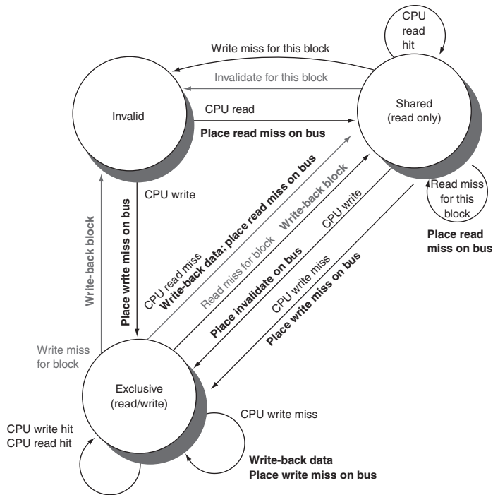
FIGURE e5.12.11 Cache coherence state diagram with the state transitions induced by the local processor shown in black and by the bus activities shown in gray. As in Figure e5.12.10 , the activities on a transition are shown in bold.
